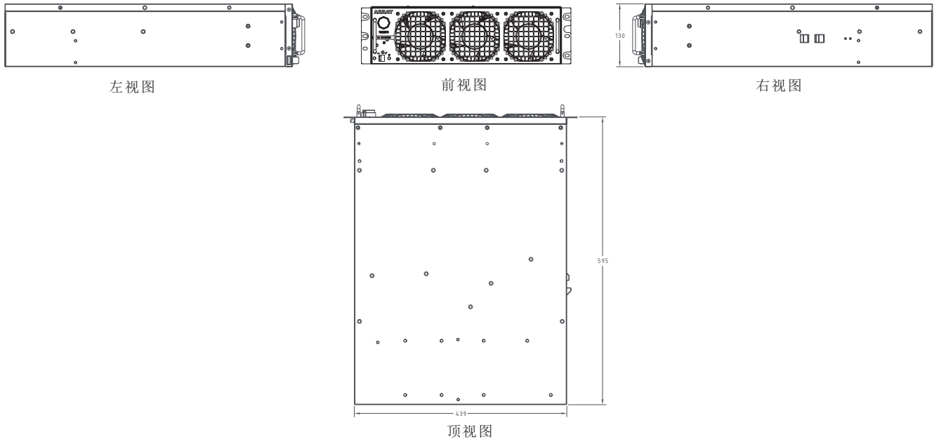
图 3-3: UPM 尺寸
