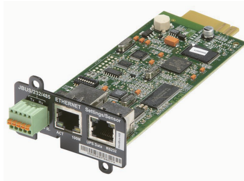
图 5-3 : Network and MODBUS Card - MS
